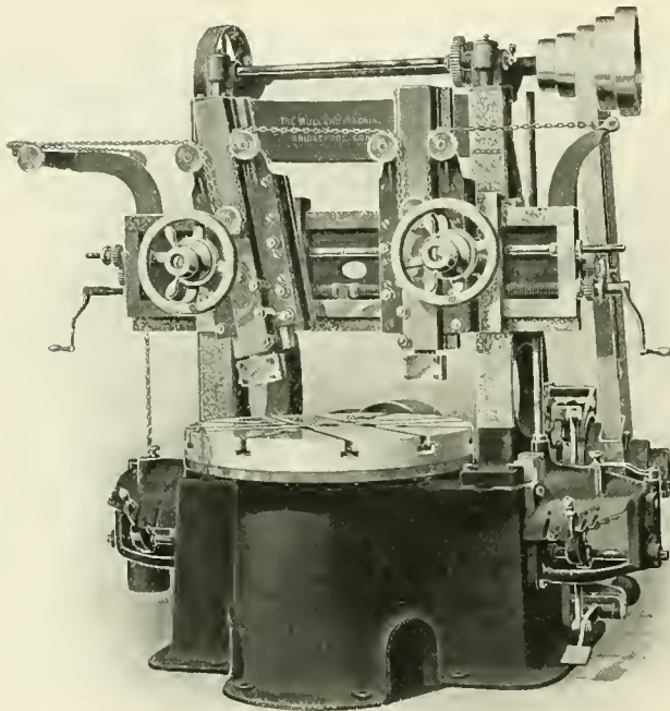
BULLARD BORING AND TURNING MILL.
